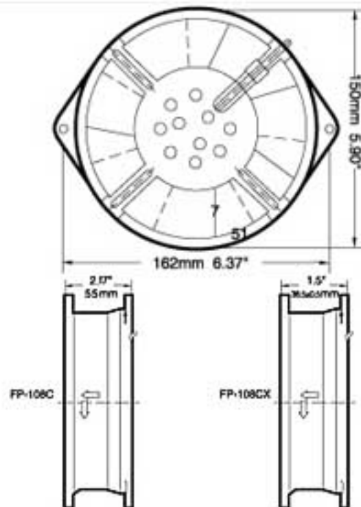
Dimensions: mm
